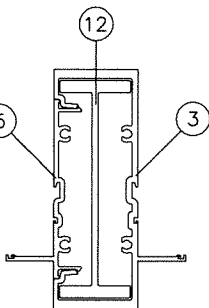
MULLION 'M2'
