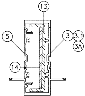
MULLION 'M4'
