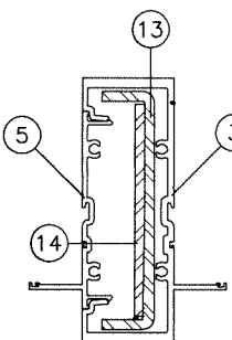
MULLION 'M4'
