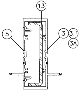
MULLION 'M3'
