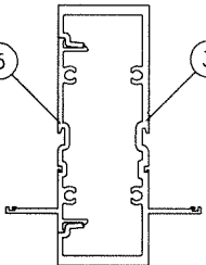
MULLION 'M1'
