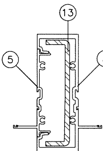
MULLION 'M3'
